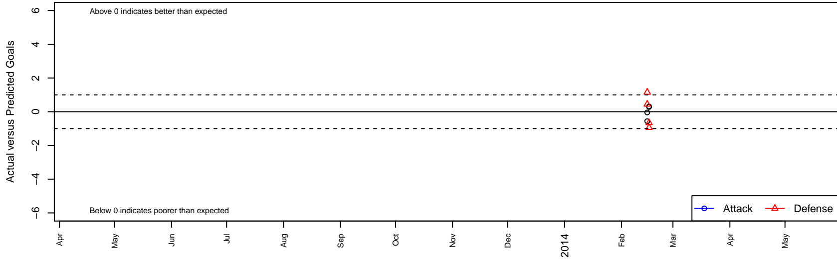
Carmel Utd SC 96 Elite B95 Dots are actual minus expected GF (blue circles) and GA (red triangles). Blue line is smoothed change in attack strength. Red is smoothed change in defense strength.
